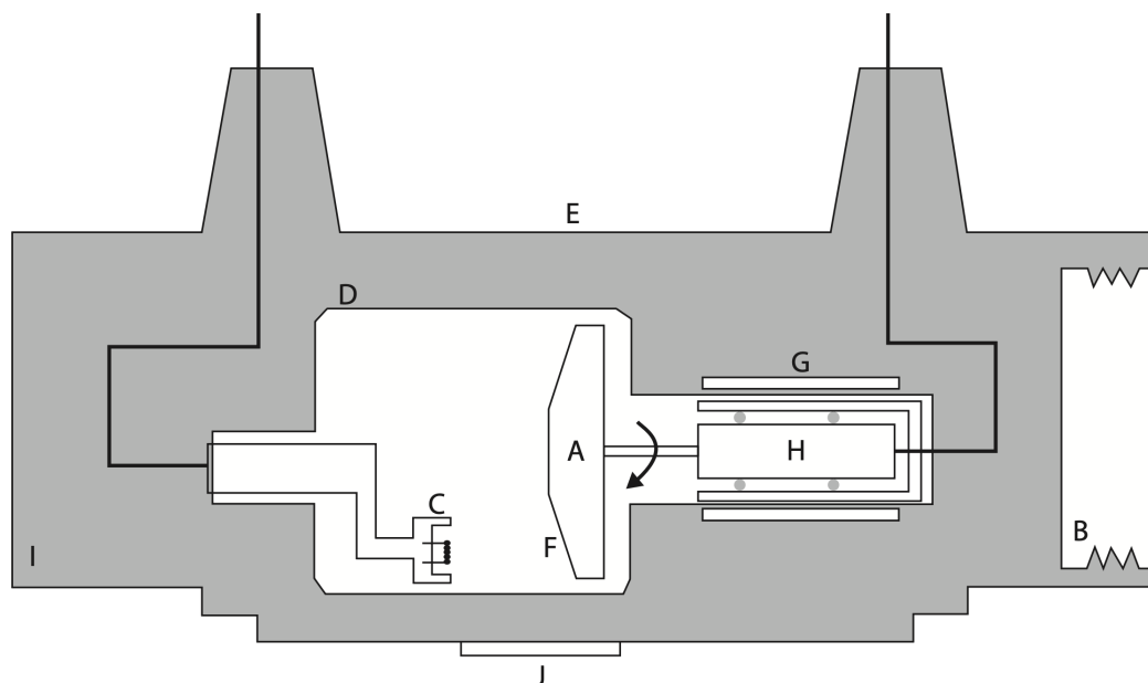
Figure 2: X-ray tube schematic diagram. A: Anode target, B: Bearing, C: Cathode filament, D: Envelope, E: Housing, F: Target, G: Stator, H: Rotor, I: Oil, J: Window [1]
